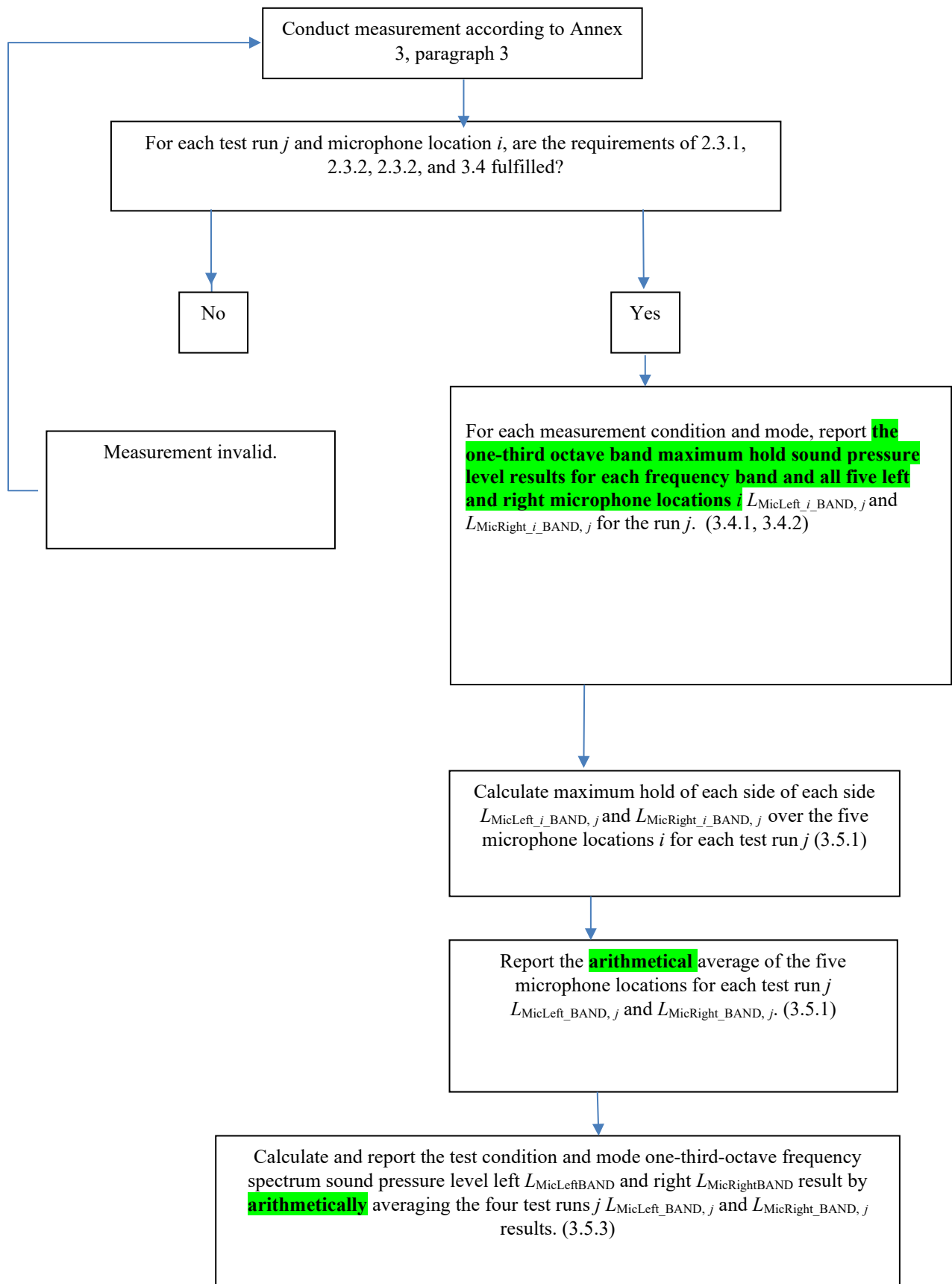
Figure 7. Flowchart for the procedure to measure and report A-weighted one third octave sound pressure levels
