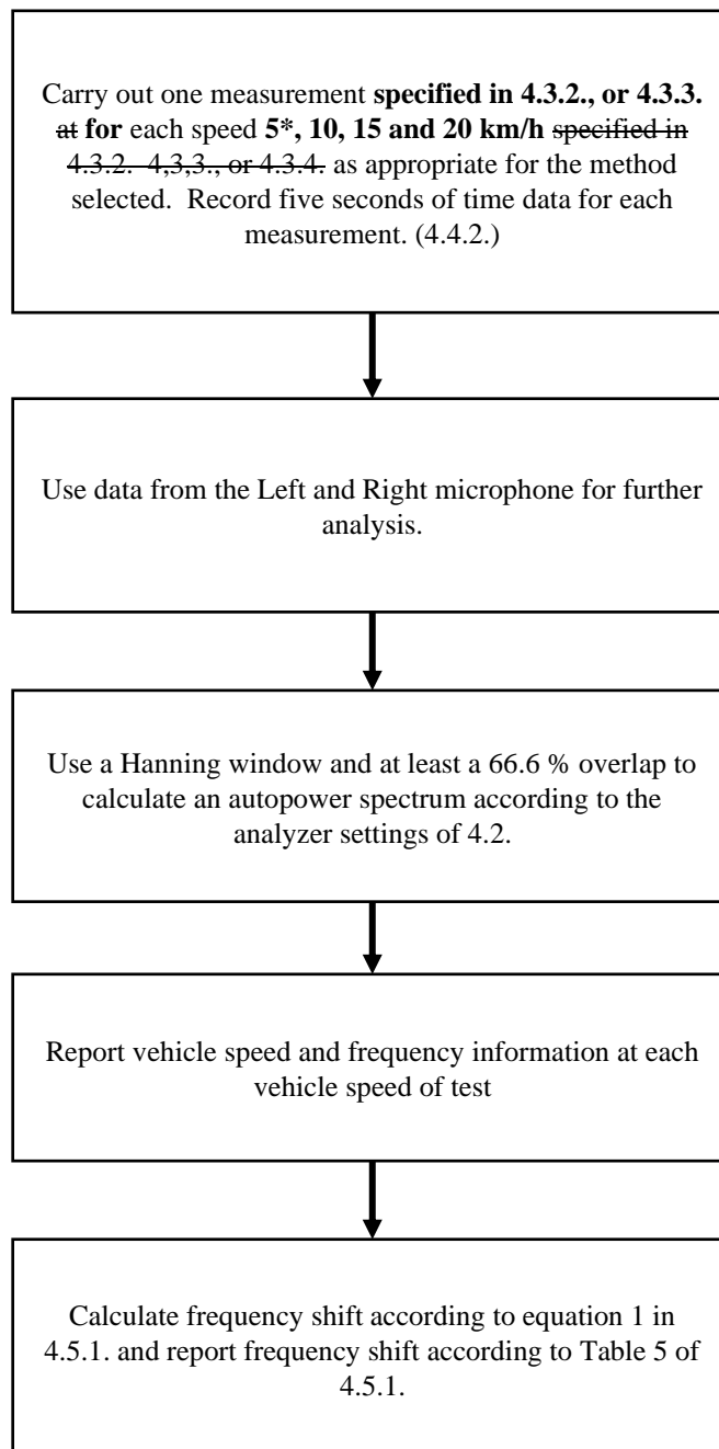
Figure 7c Test procedures for measurement of frequency shift, Methods B, C and D and E
