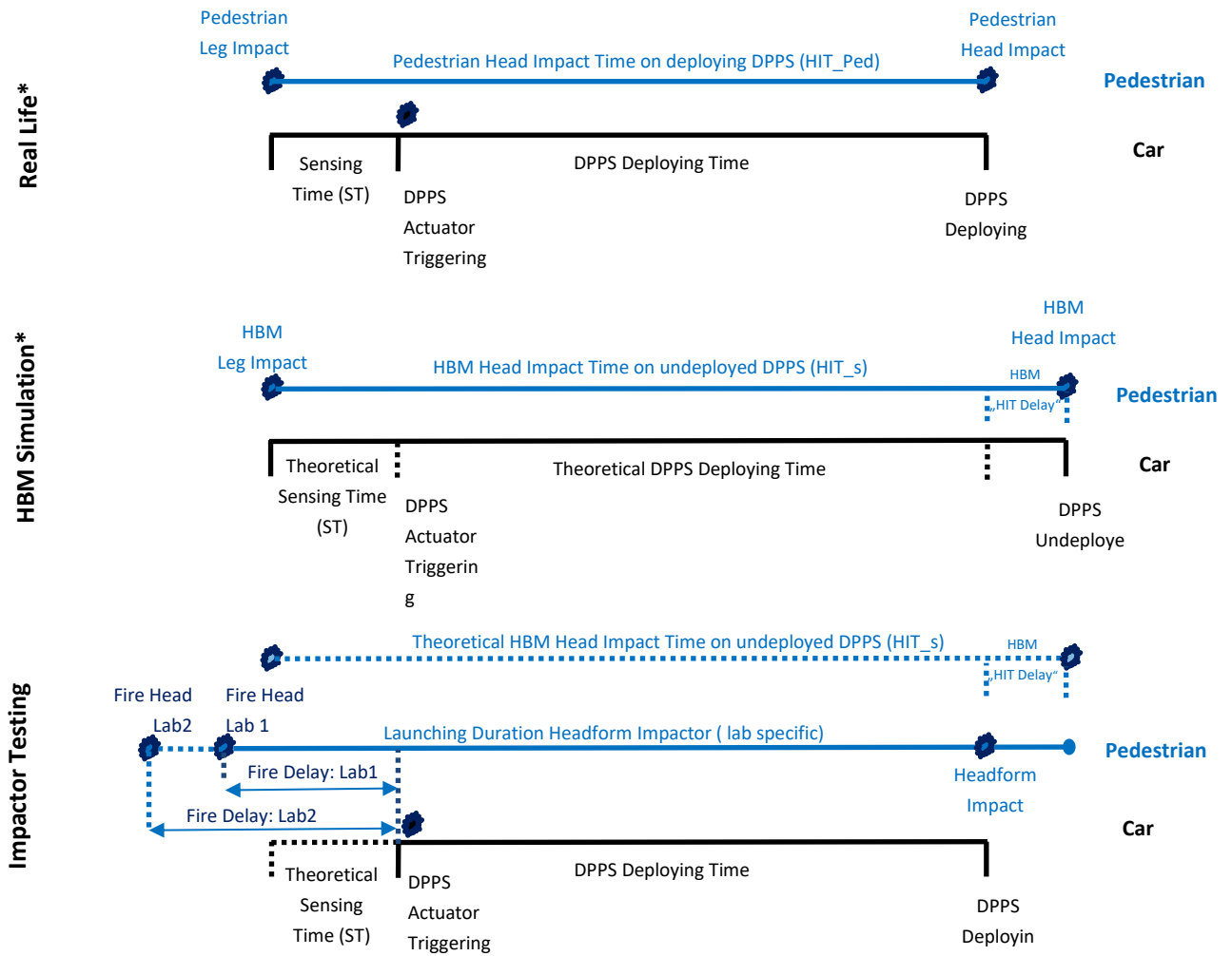
Figure 1 (a) Transfer of real life accident situation with deploying DPPS to ambient conditions for impactor testing.
