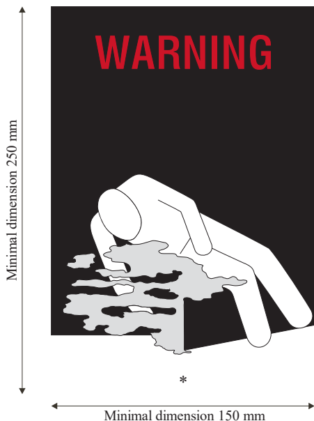
Figure 5.5.2: Asphyxiation warning mark for cargo transport units
