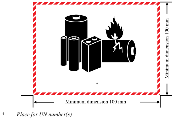
Figure 5.2.5: Lithium or sodium ion battery mark
