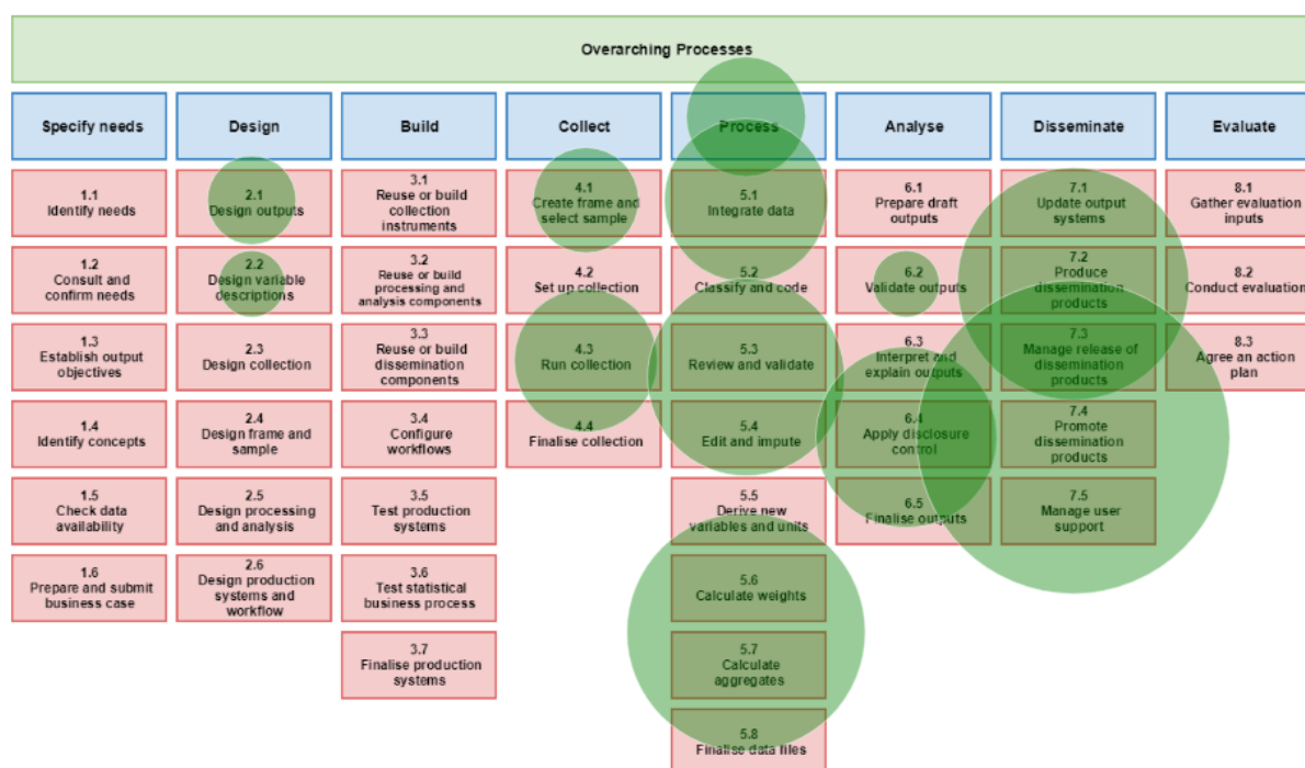
Figure 1 Awesome official statistics packages organized by GSBPM
