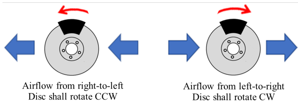
Figure 8.6. Schematic representation of disc rotation viewed from the wheel side (road side)
