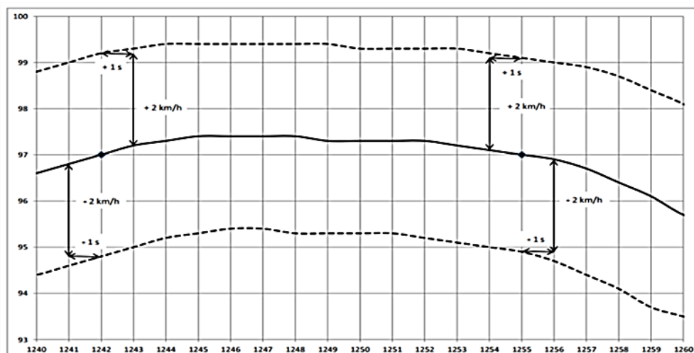
Tolerance limits for speed violations during the WLTP-Brake cycle
