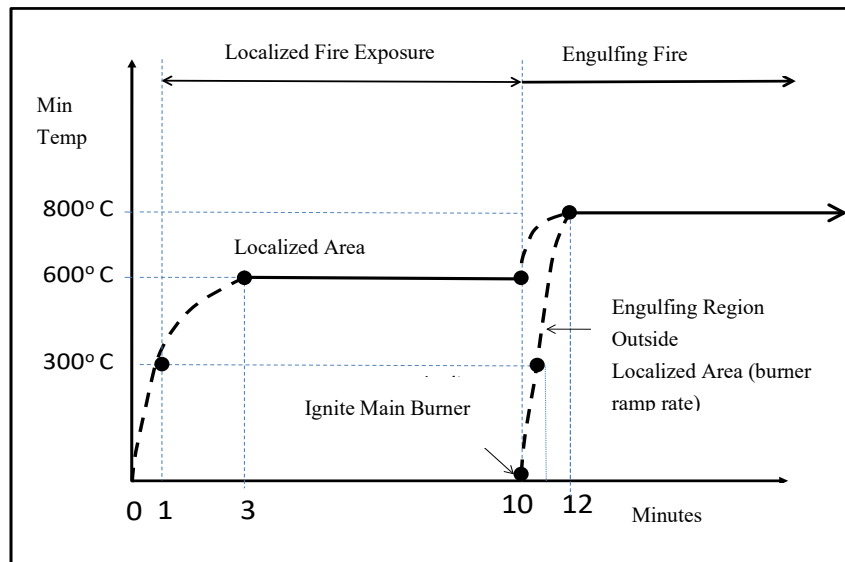
Figure 4 Temperature Profile of the Fire Test
