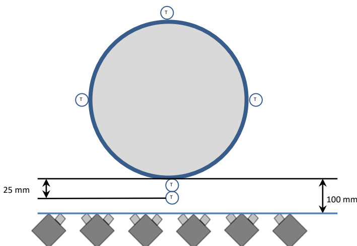
Figure 7 Position the Bottom of the Container Relative to the Burner
