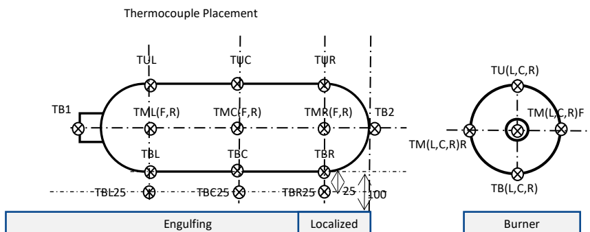
Figure 5 Example of the Placement of Instrumentation on the Pre-Test Cylinder
