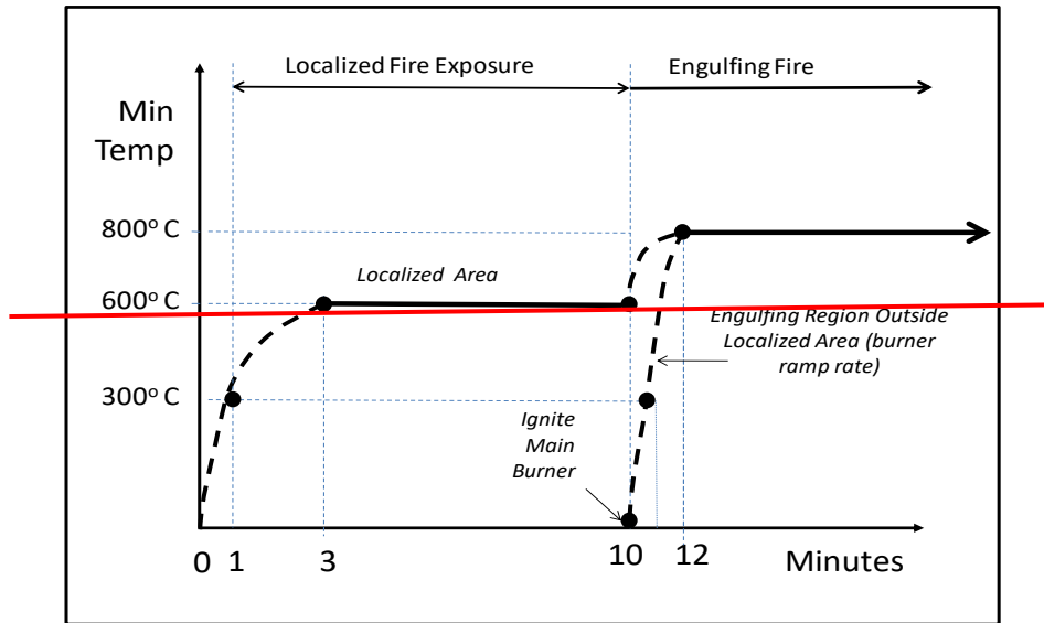
Figure 711 Temperature profile of fire test
