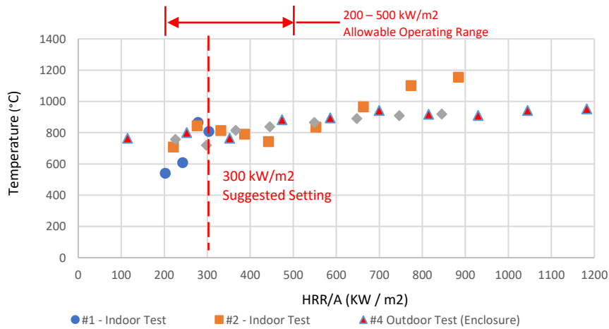
Figure 22 Temperature of burner monitor during thermal mapping of localized burner
