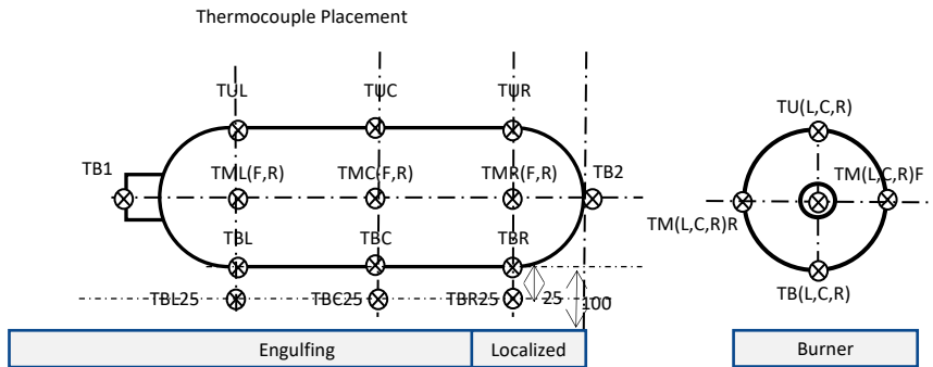
Figure 7 Example of Placement of Instrumentation on the Pre-Test Cylinder
