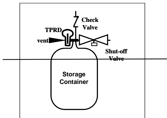
Figure 1 Typical compressed hydrogen storage system
