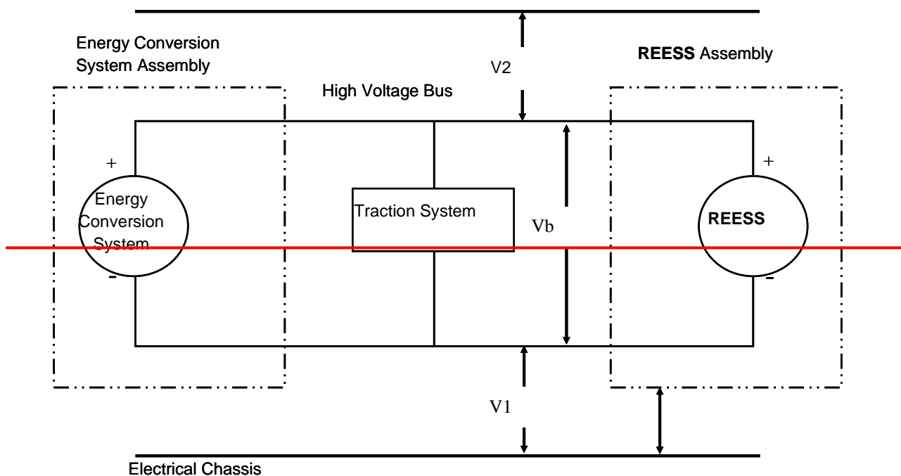
Figure 13 Measurement of V_b , V_1 , V_2
