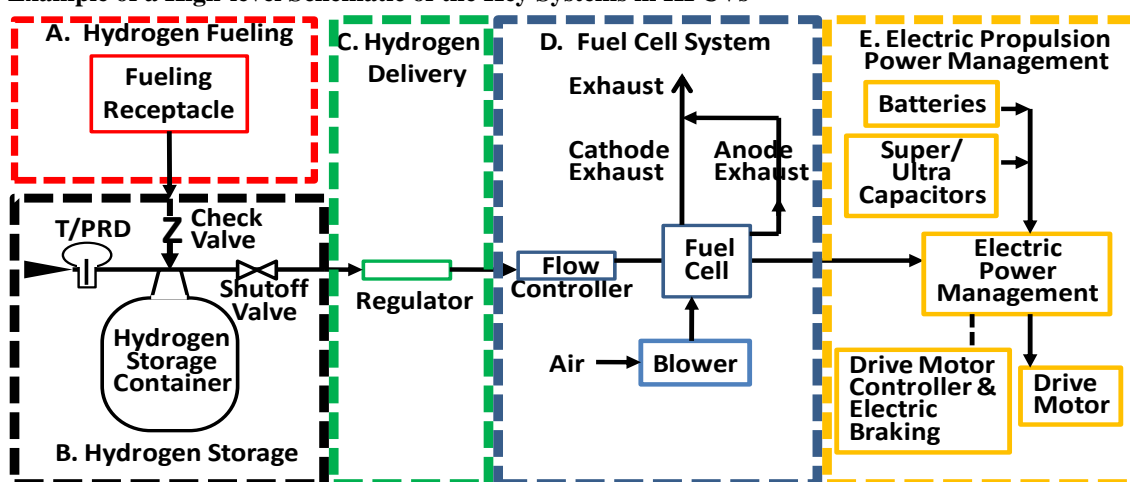
Example of a High-level Schematic of the Key Systems in HFCVs
