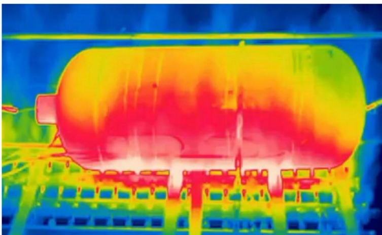
Figure 27 Example of the Thermal Imaging Results for the Prescribed Burner Configuration
