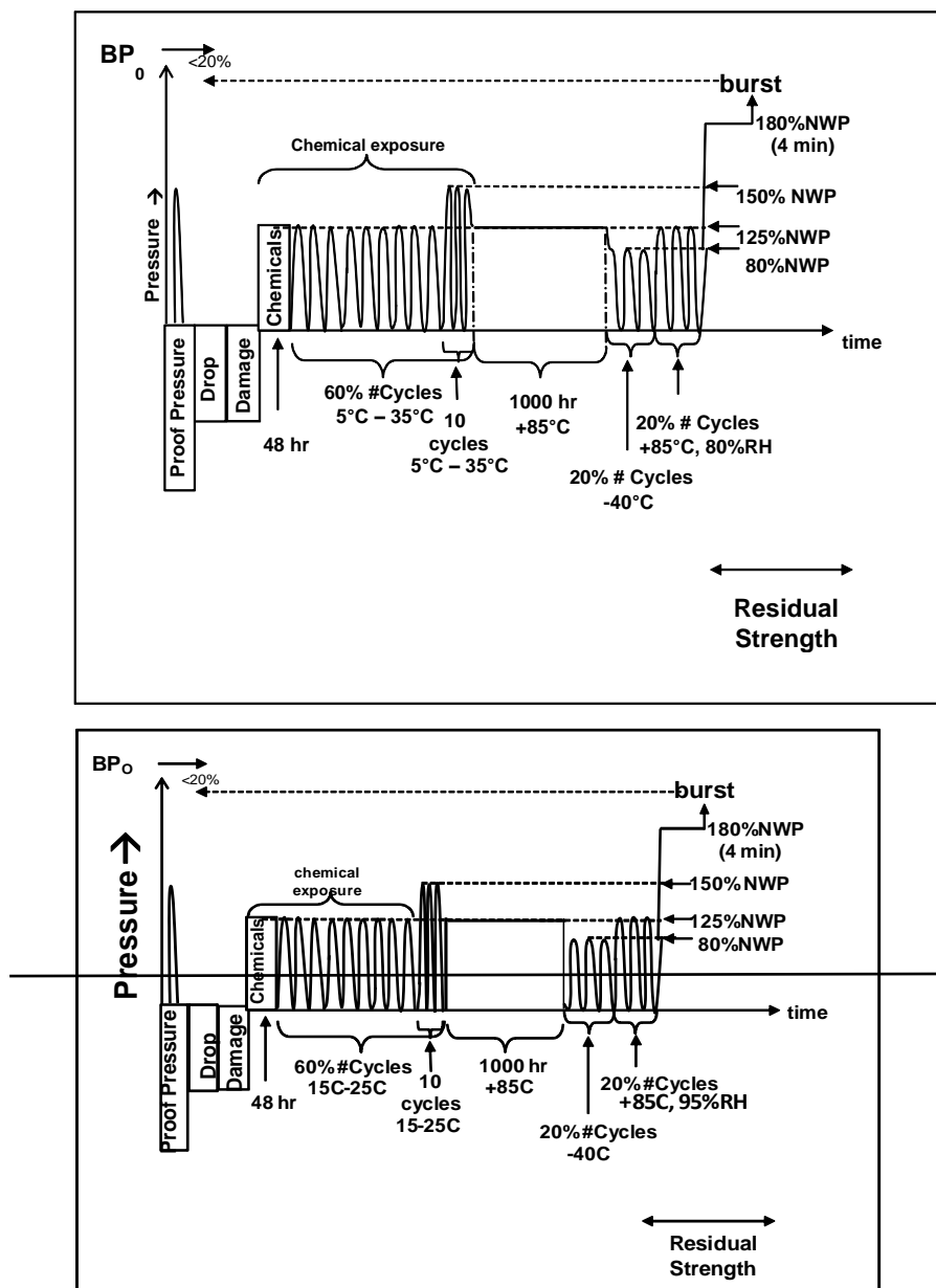
Figure 12 Verification test for performance durability (hydraulic)
