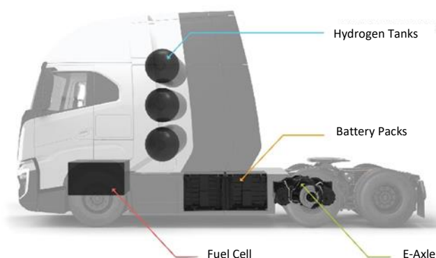
Figure 4 Example of a hydrogen fuel cell truck
