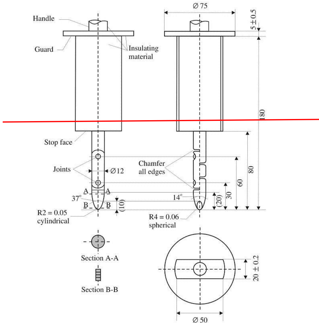
Figure 11 Jointed Test Fingers
