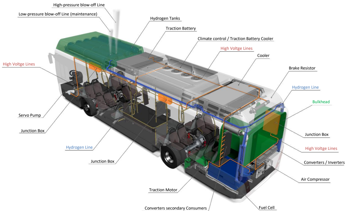
Figure 3 Example of a hydrogen fuel cell bus
