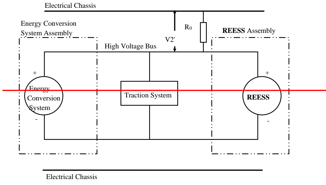
Figure 10 Measurement of V_2
