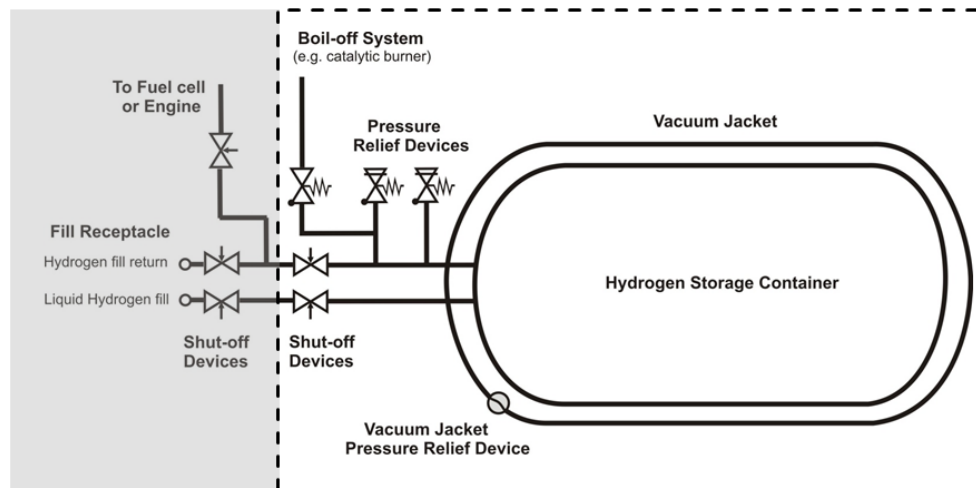
Figure 367 Typical Liquefied Storage System
