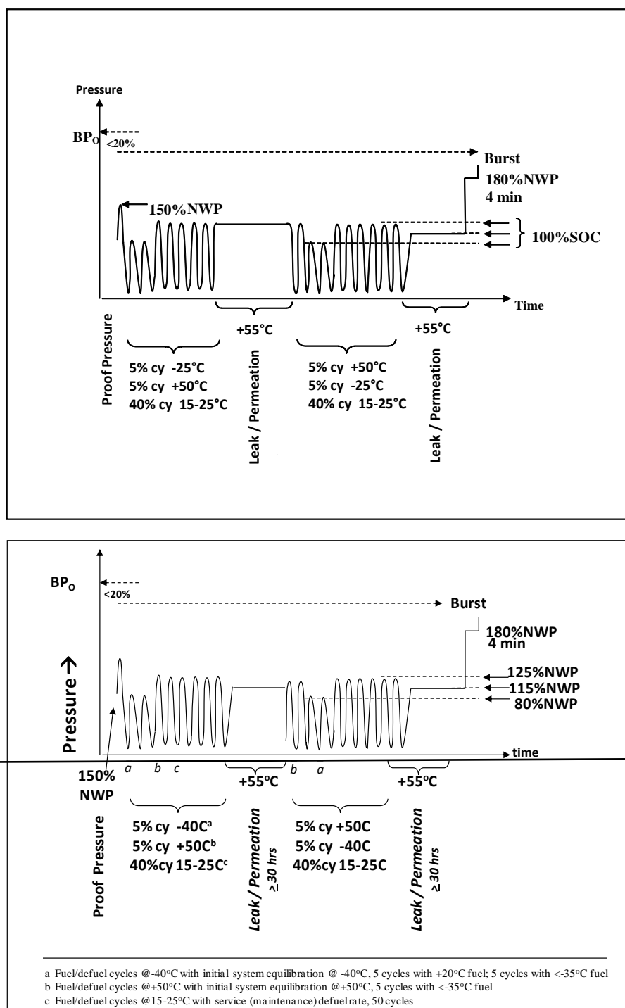
Figure 23 Verification Test for Expected On-Road Performance (Pneumatic/hydraulic)
