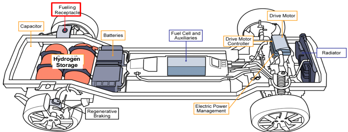
Figure 2 Example of a Hydrogen Fuel Cell Vehicle-Passenger Car
