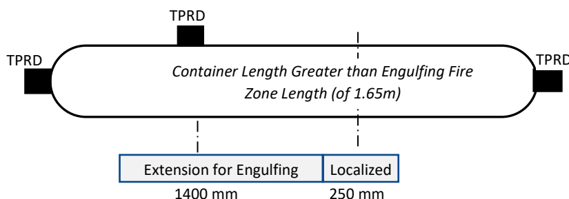
Figure 35 Engulfing Burner Configuration when the Localized Fire Zone is Located at the Maximum Distance from Multiple TPRDs
