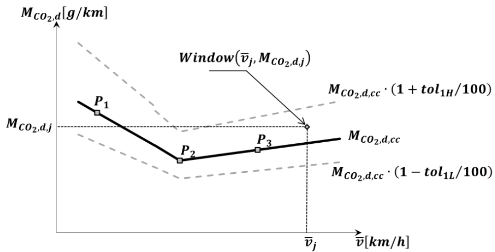
Figure A8/3 Vehicle CO 2 characteristic curve and tolerances for ICE and NOVC-HEV vehicles
