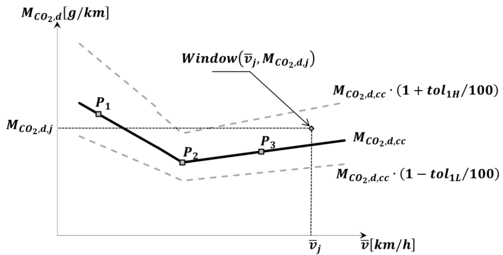
Figure A8/3 Vehicle CO 2 characteristic curve and tolerances for ICE and NOVC-HEV vehicles
