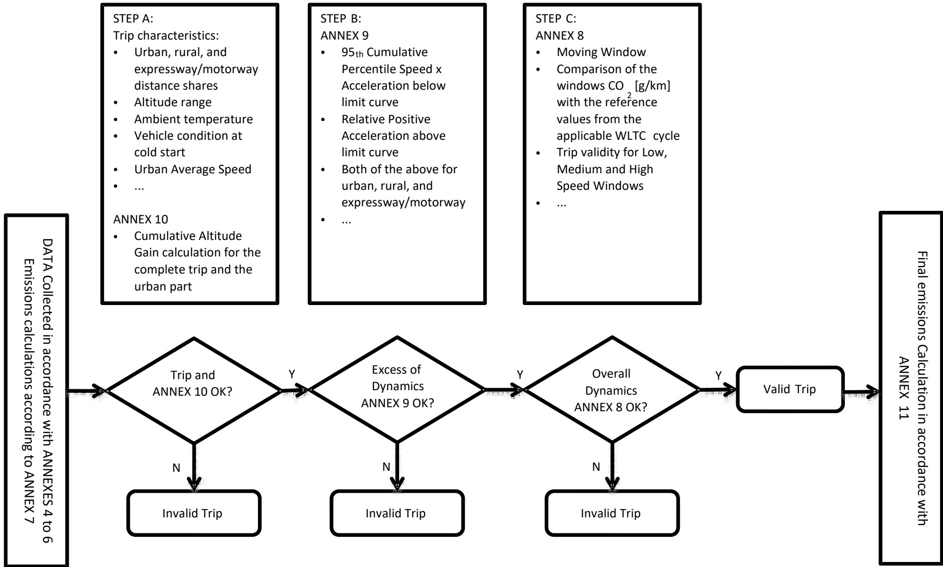
Figure 6 Assessment of trip validity – schematic (i.e. not all details are included in the steps included in the figure, see the relevant annexes for such details)
