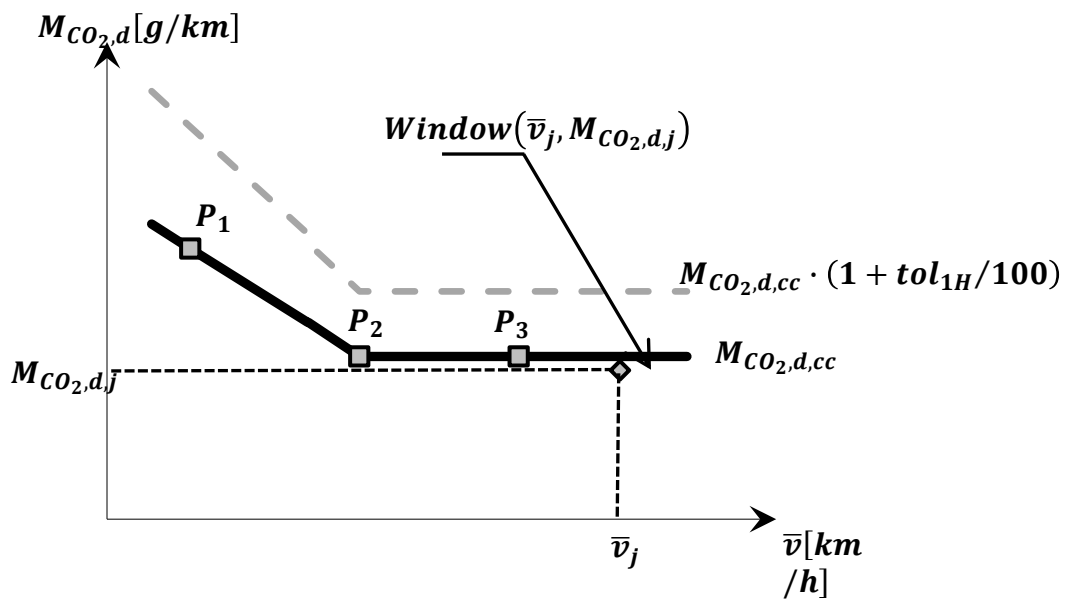
Figure A8/4-2 Vehicle CO 2 characteristic curve and tolerances for OVC-HEV vehicles for 3-phase WLTP
