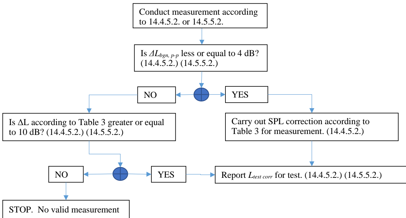
Figure 2 Vehicle A-weighted sound pressure level measurement correction criteria
