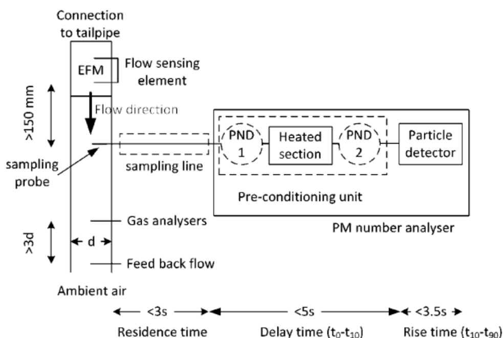
Example of a PM number analyser setup
