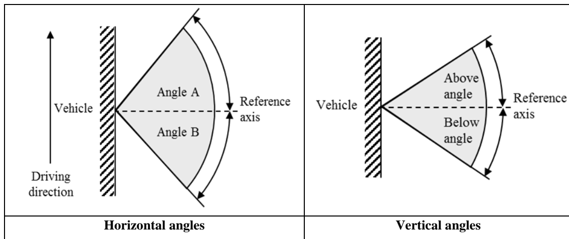
Angles of geometric visibility, horizontal and vertical
