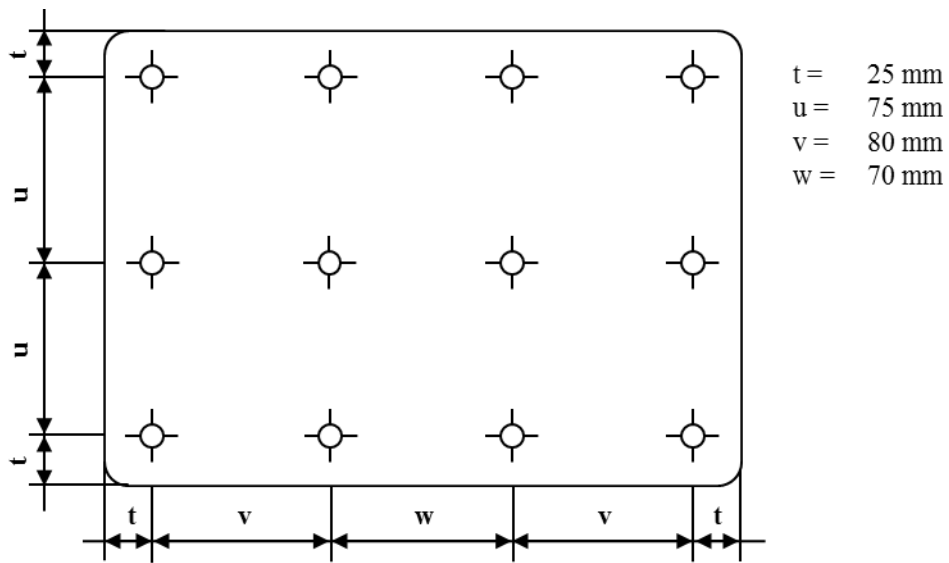
Measuring points for plate size 280 x 200 mm
