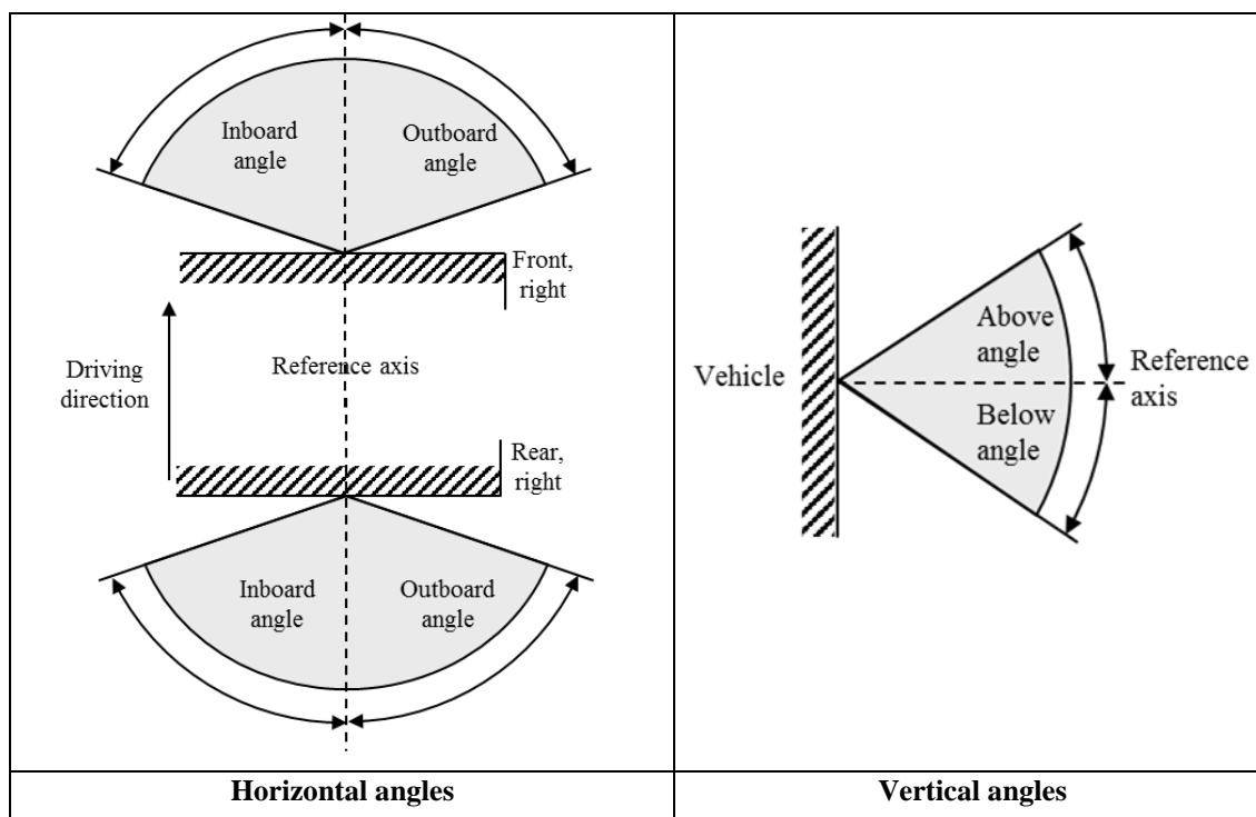
Figures A2-I: Angles of geometric visibility, horizontal and vertical
