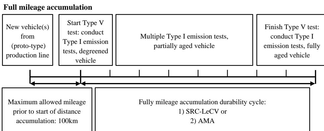
Figure 1 Test Type V – Durability test procedure with full mileage accumulation
