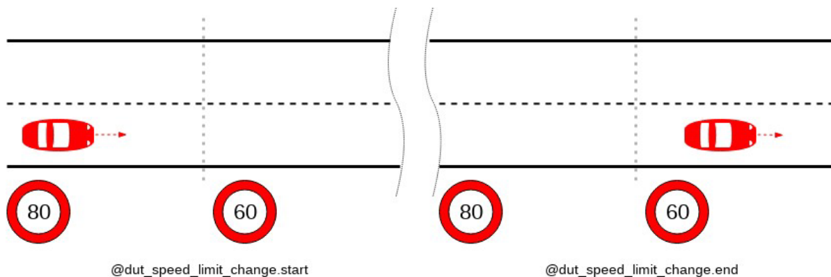
Ego vehicle speed limit change scenario
