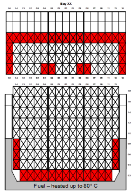
Figure 514 - Positioning flexitanks
