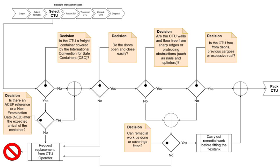
Figure 244 – Flexitank transport process - CTU Selection
