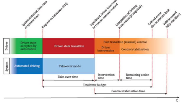
Figure 2 — System-initiated transition from automated to manual driving
