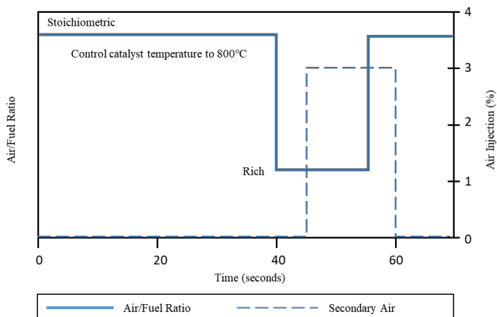
Figure A4/1 Standard bench cycle (SBC)
