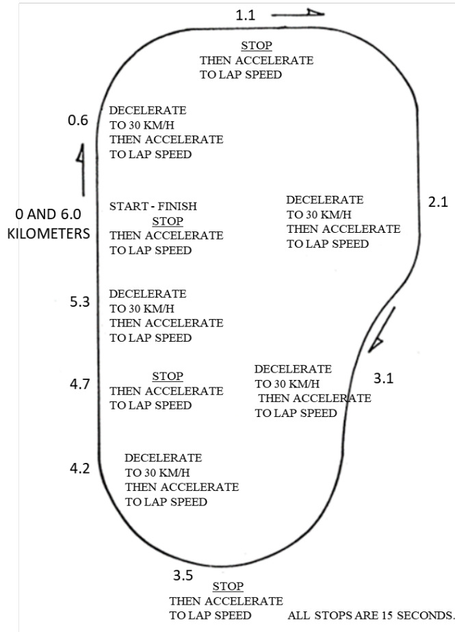
Figure A2/1 Driving schedule AMA test sub-sub-cycle
