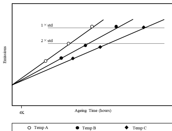
Figure A4/2 Catalyst Ageing
