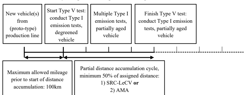
Figure 2 Test Type V – Durability test procedure with partial distance accumulation
