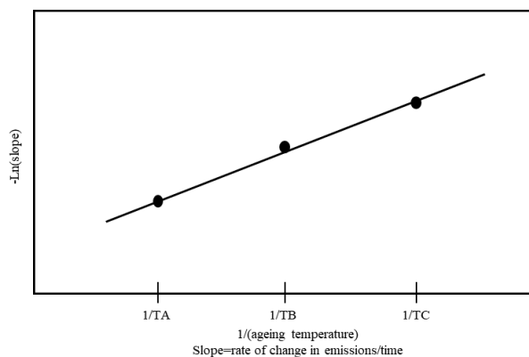
Figure A4/3 Determining the R-factor
