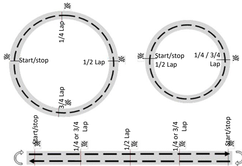
Figure A1/1 Simplified representation of possible test track configurations
