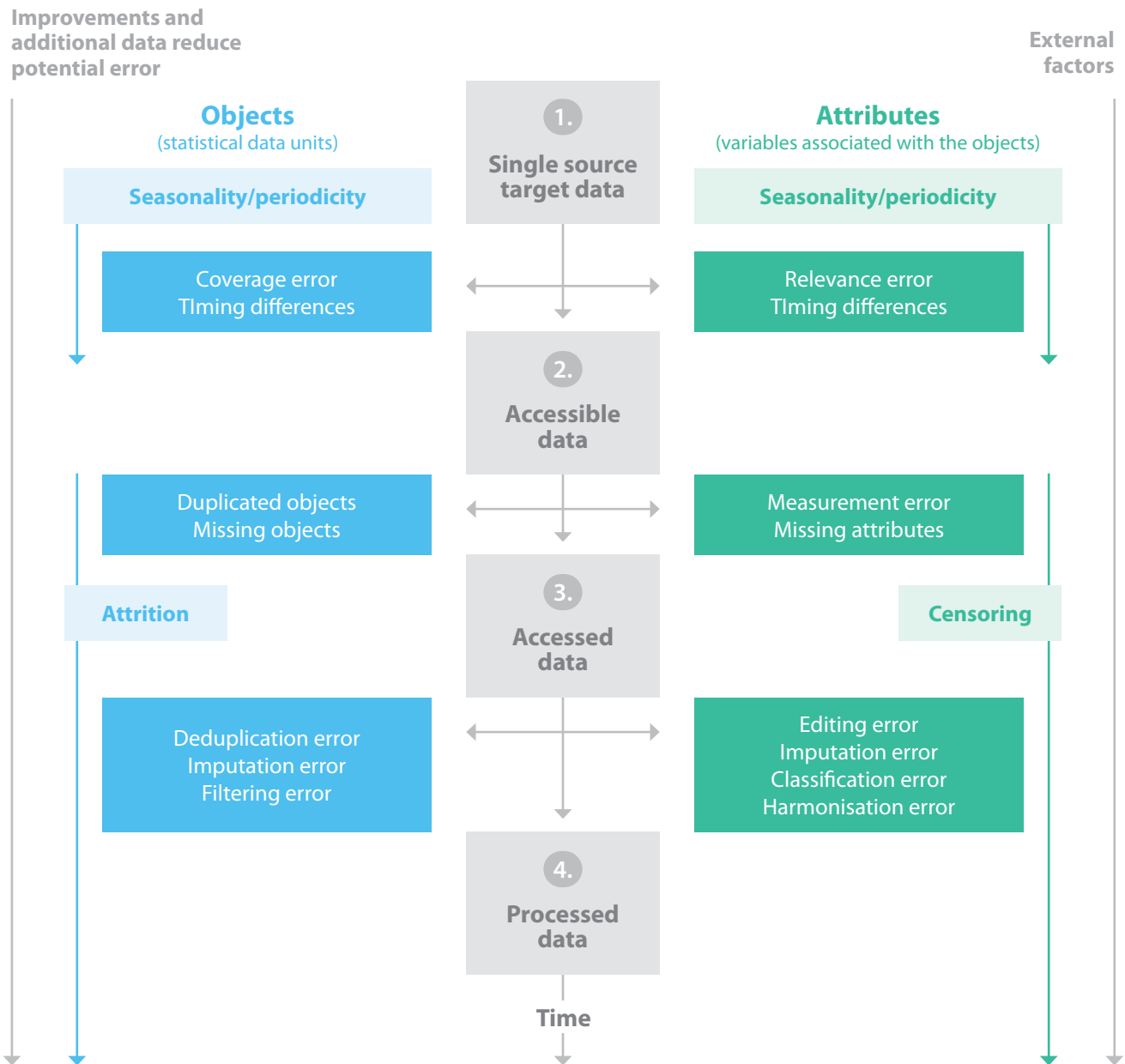
FIGURE 5: SINGLE SOURCE ERROR FRAMEWORK
