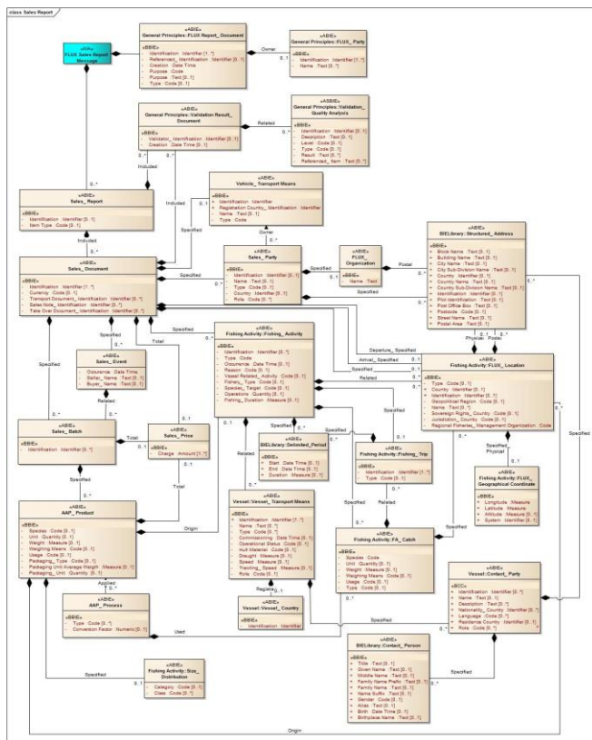
Figure 8: class diagram Sales Report Message
