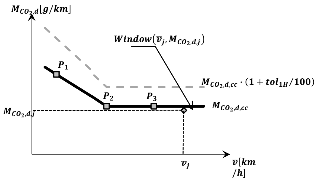
Figure A8/4-2 Vehicle CO 2 characteristic curve and tolerances for OVC-HEV vehicles for 3-phase WLTP
