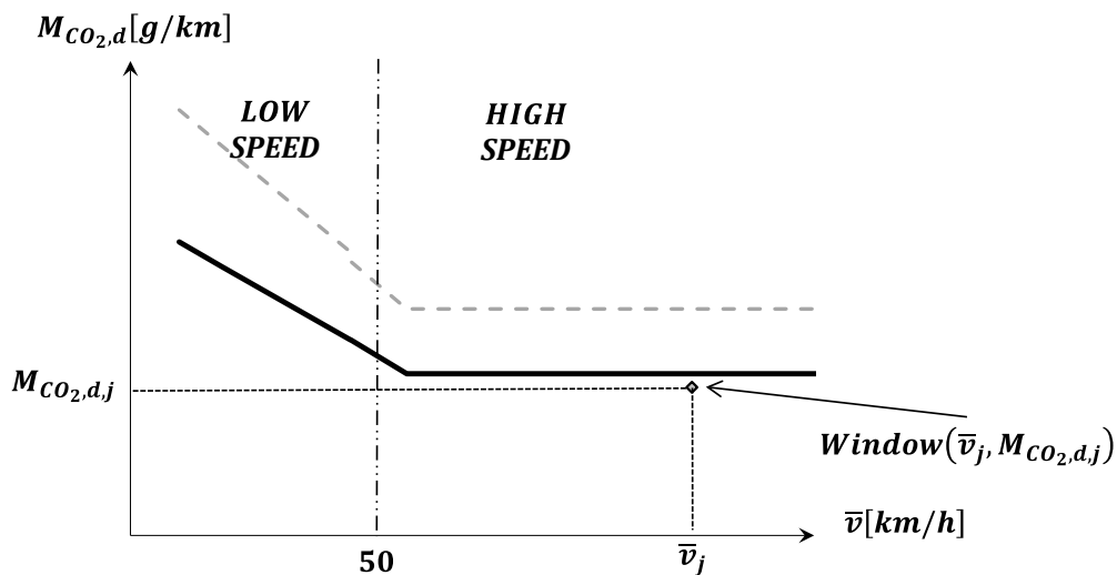
Figure A8/6-2. Vehicle CO 2 characteristic curve: low and high speed driving definitions (Illustrated for OVC-HEV vehicles)
