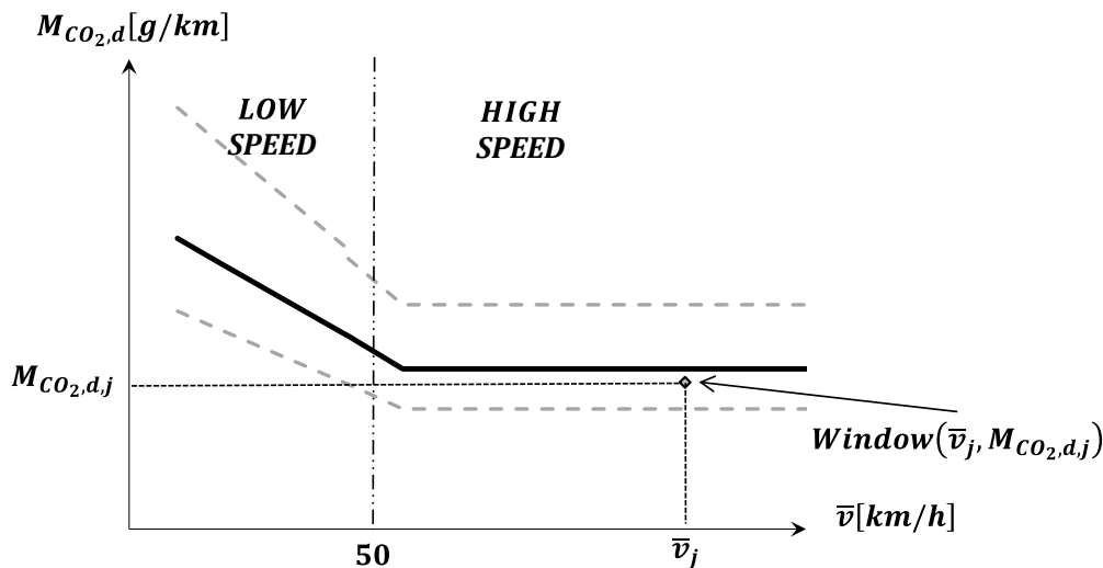
Figure A8/5-2 Vehicle CO 2 characteristic curve: low and high speed driving definitions (Illustrated for ICE and NOVC-HEV vehicles)
