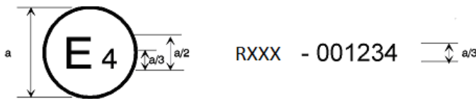
Figure 1 (see paragraph 4.2. of this Regulation)
