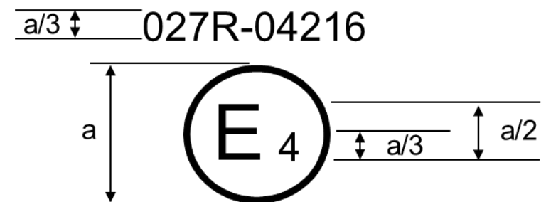
Figure A24-V: Arrangement of the approval mark for advance warning triangle
