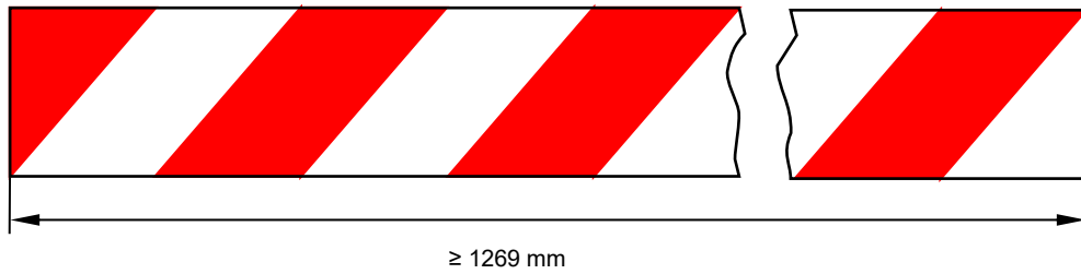
Figure A5-IV: Retro-reflective material marking of Class 5
