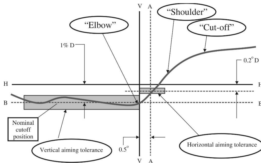
Figure A5-I Visual aiming of the cut-off
