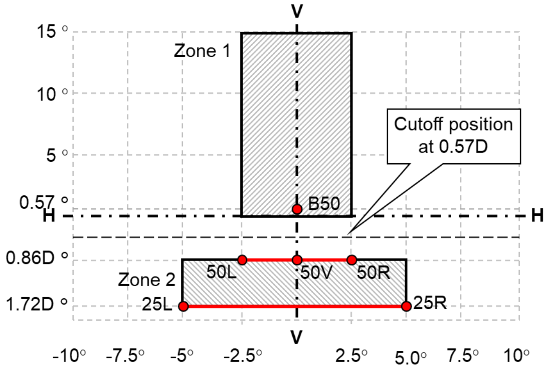
Figure A4-IX Passing beam test points and zones for Class BS headlamp(s)
