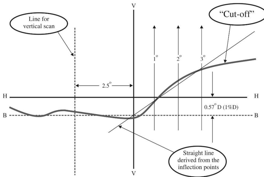
Figure A5-IV Instrumental vertical and horizontal adjustment - Three line scan method
