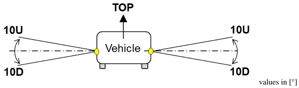
Figure A4-XIV Vertical geometric visibility for cornering lamps
