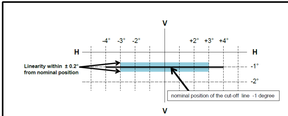
Figure A6-II Shape and position of the “cut-off” line of the front fog lamp
