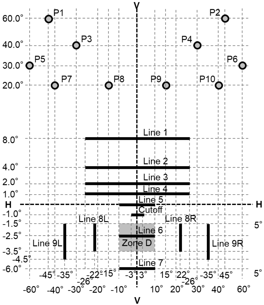
Figure A4-XI Light distribution of the Class F3 front fog lamp
