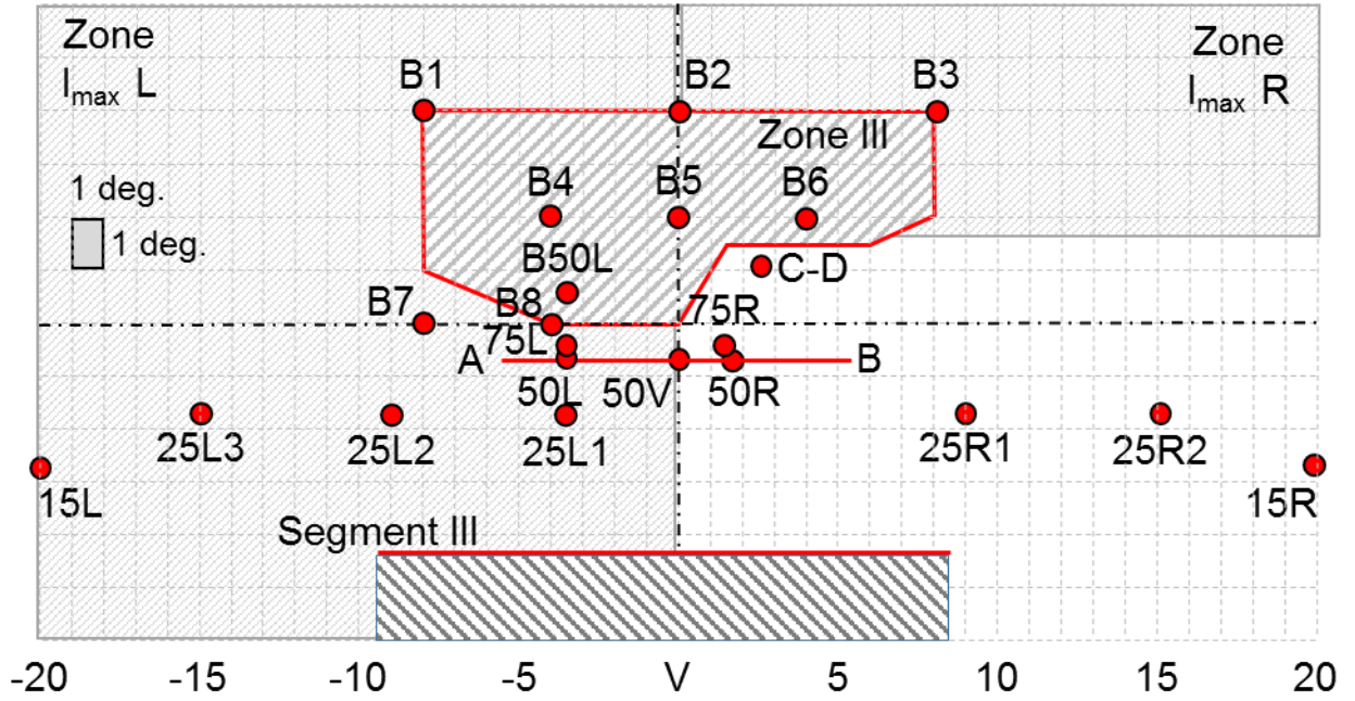
Figure A4-VI Passing beam with gas discharge light sources for right-hand traffic
