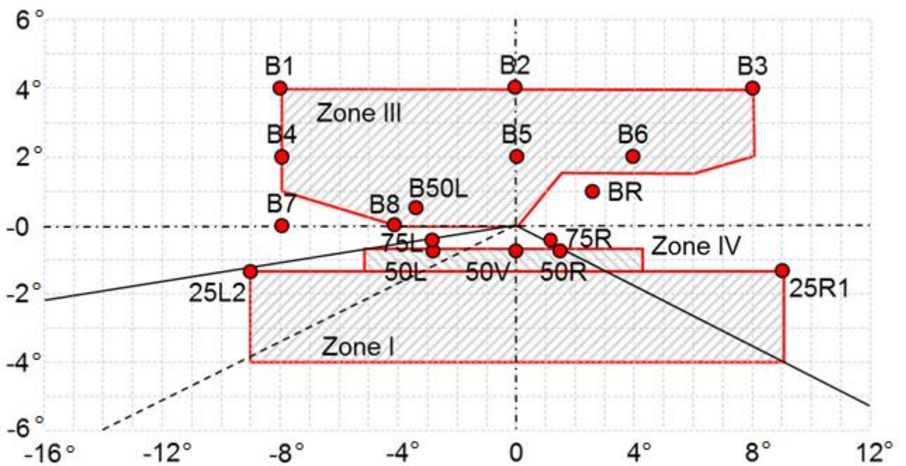
Figure A4-V Passing-beam for right-hand traffic
