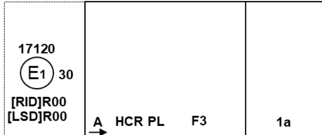
Figure A13-IV Marking example 4
