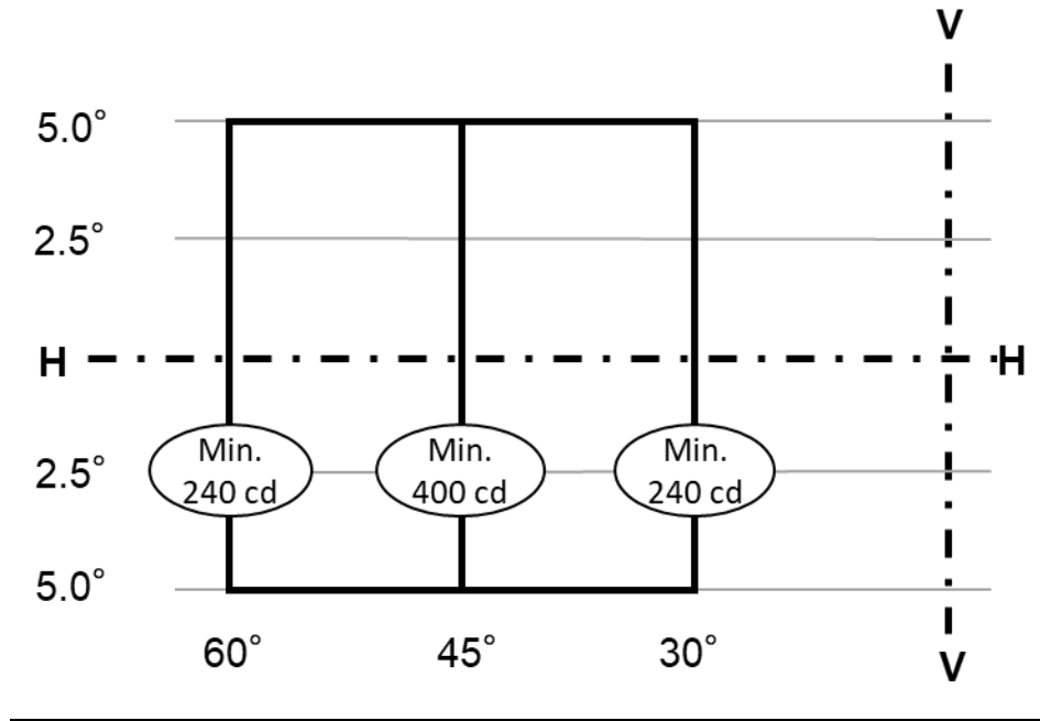
Figure A4-XIII Horizontal geometric visibility for cornering lamps
