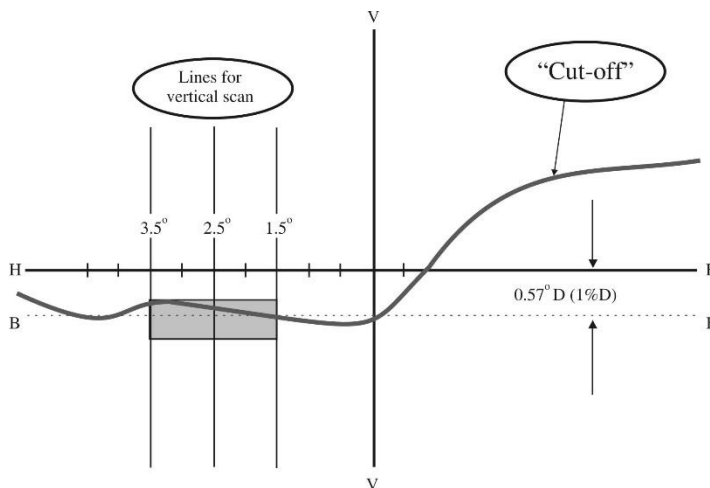
Figure A5-II Measurement of "cut-off" quality
