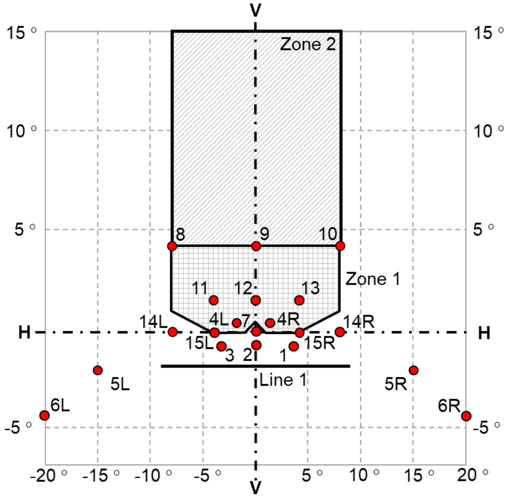
Figure A4-X Passing beam - position of test points and zones for Classes CS, DS and ES headlamp(s)
