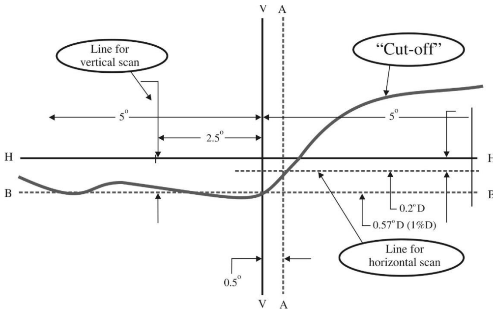
Figure A5-III Instrumental vertical and horizontal adjustment - horizontal line scan method
