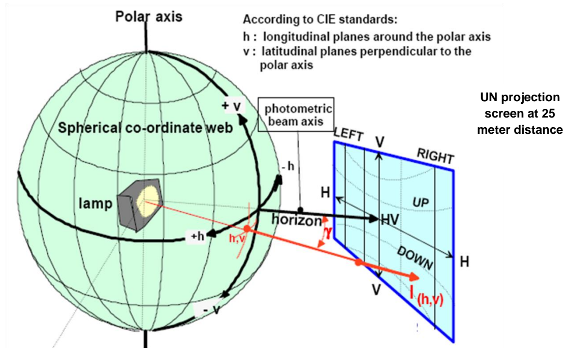
Figure A4-I Spherical coordinate measuring system
