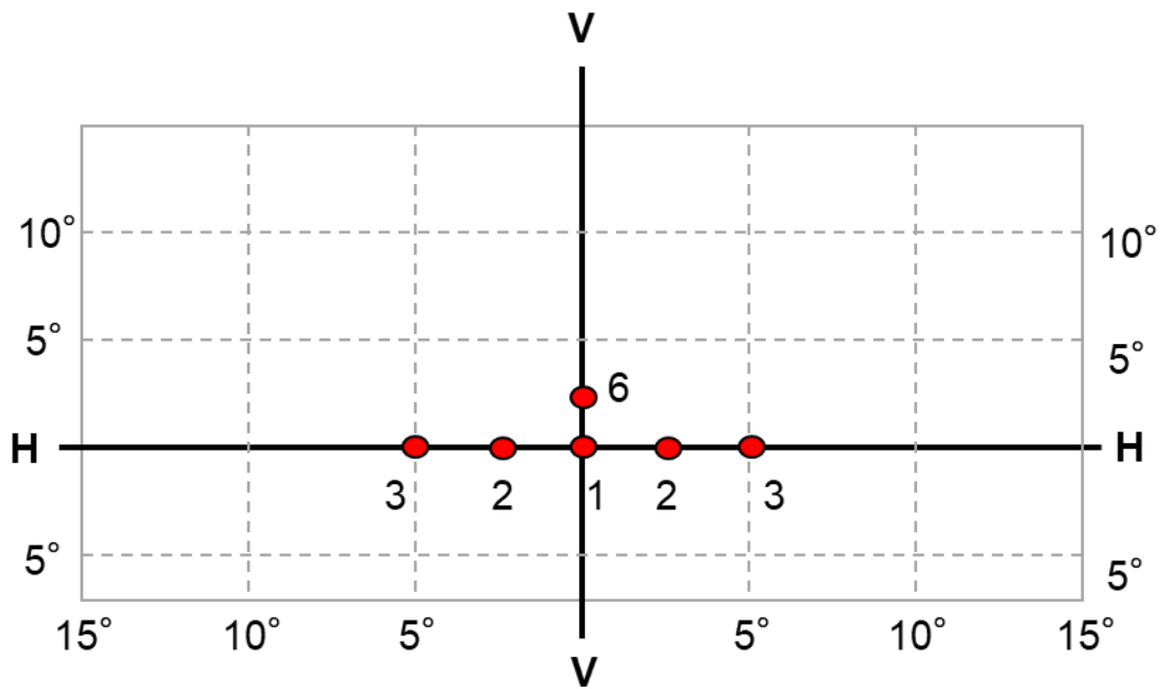
Figure A4-IV Secondary driving beam - position of test points
