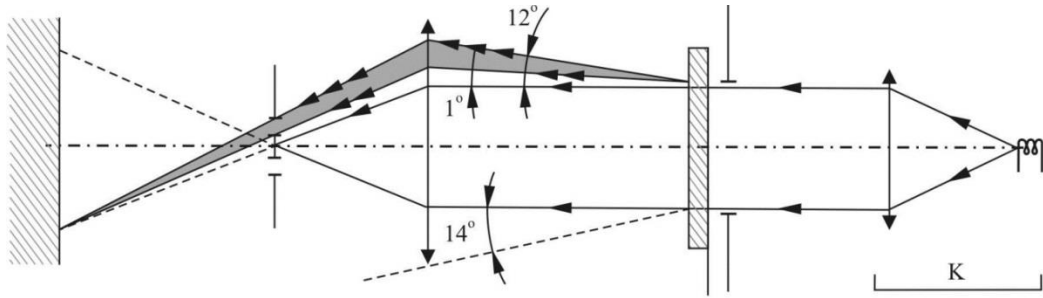
Figure A8-I Optical set up for measurement of variations in diffusion and transmission
