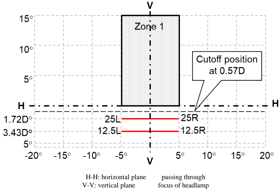
Figure A4-VIII Passing beam test points and zones for Class AS headlamp(s)
