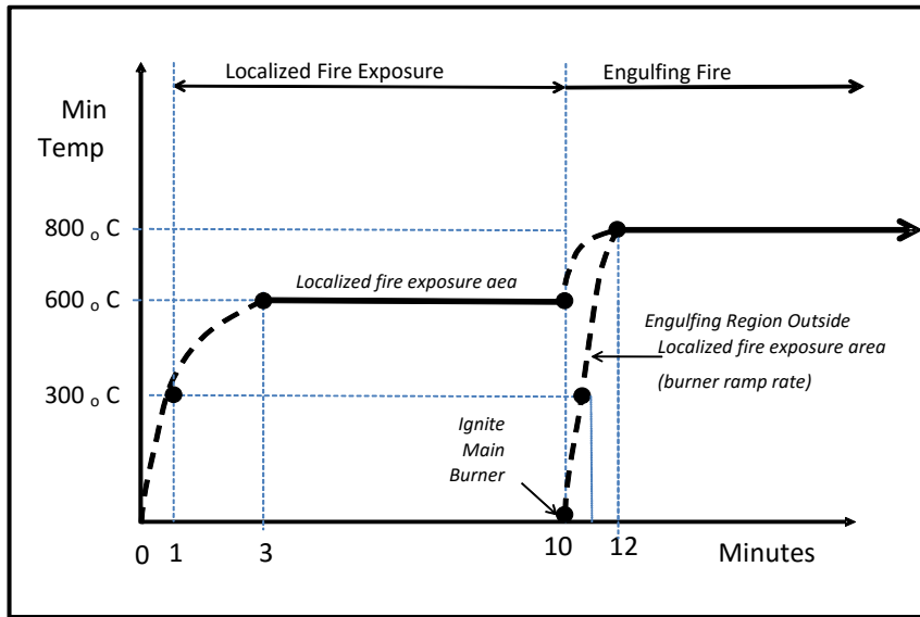
(c) Engulfing portion of the fire test
