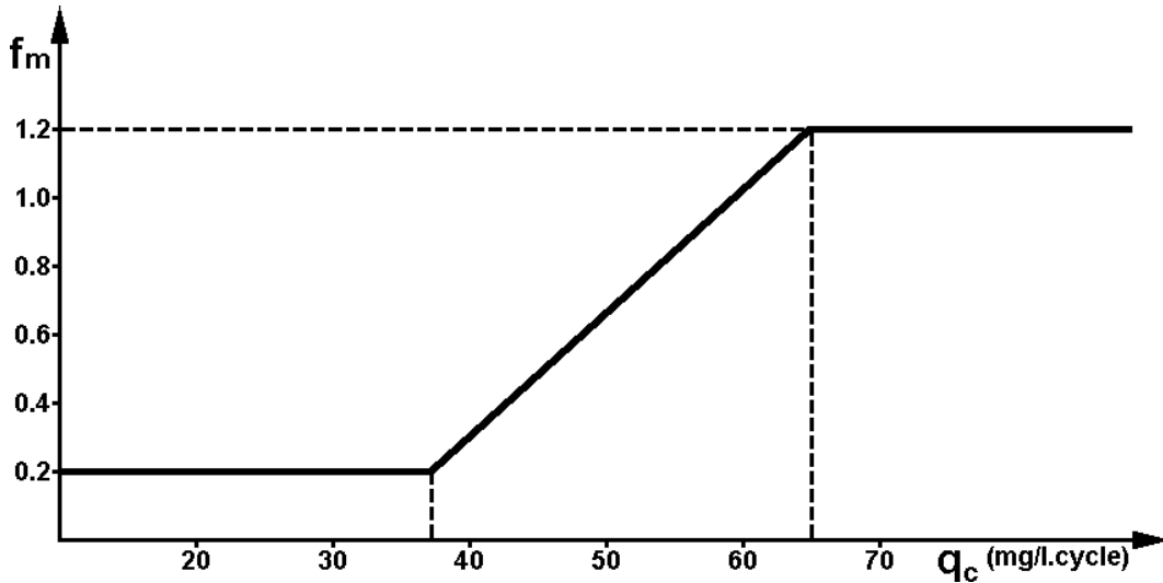
Figure 1 Determination of engine factor f_m
