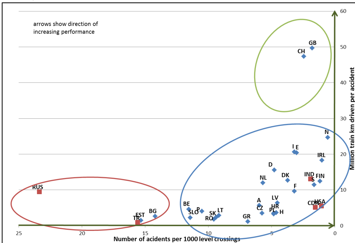
Figure 11 Safety assessment of level crossings, significant accidents to number of level crossings versus million train kilometers driven per accident, “ERA” and “other” countries, 2014
