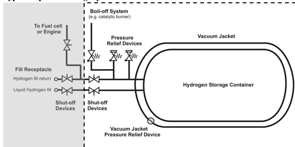
Typical liquefied storage system
