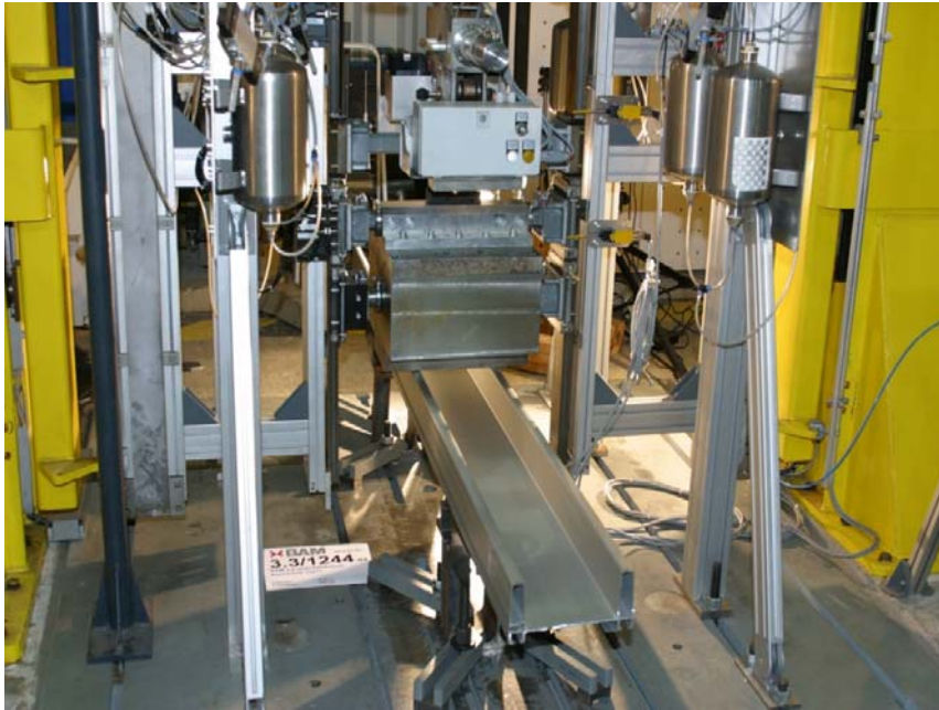
Figure 4: Test setup for dynamic tests at the guided drop test stand
