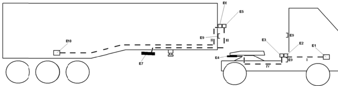
Figure A: Point-to-point connection ECU Tractor (E1) and ECU Trailer (E10) via ACV
