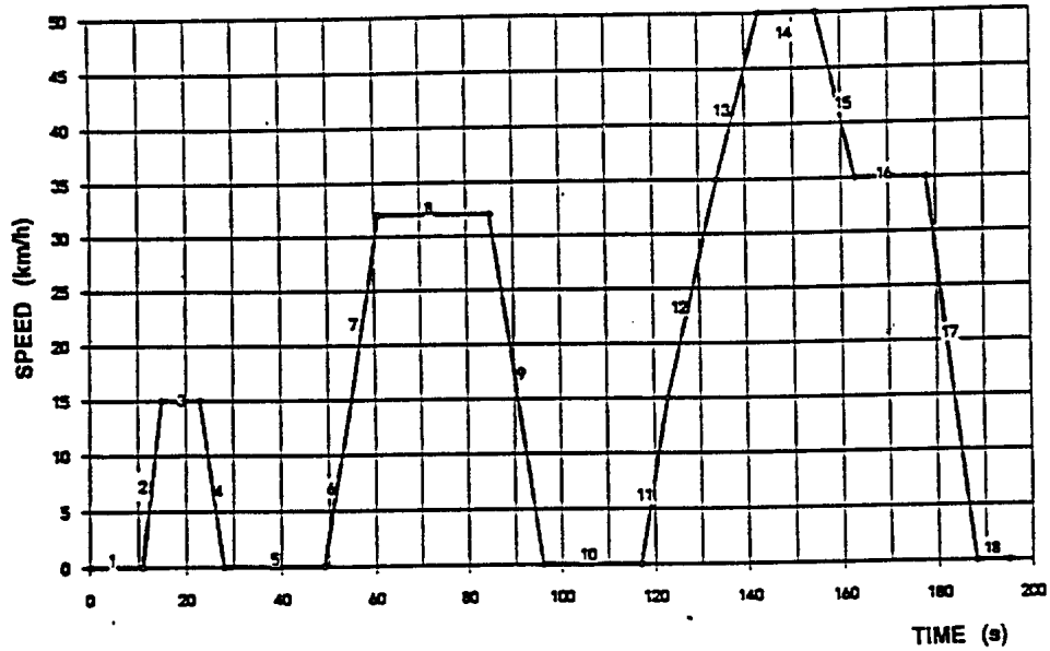
Figure 2 Elementary urban cycle (195 seconds)
