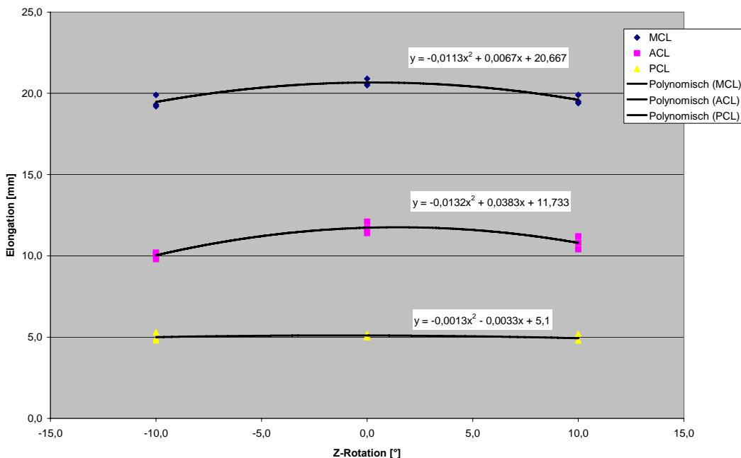
Fig. 12: Rotation around Z-axis: Knee elongations
