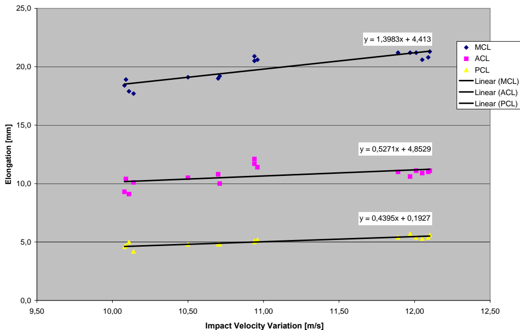
Fig. 16: Impact velocity variation: Knee elongations
