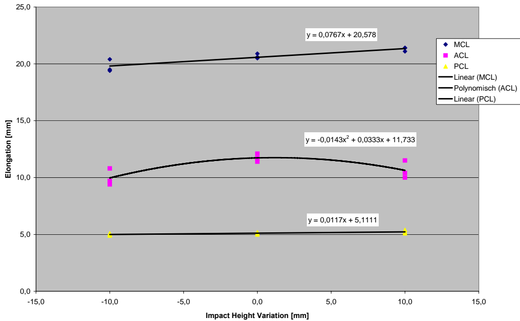
Fig. 14: Impact height variation: Knee elongations
