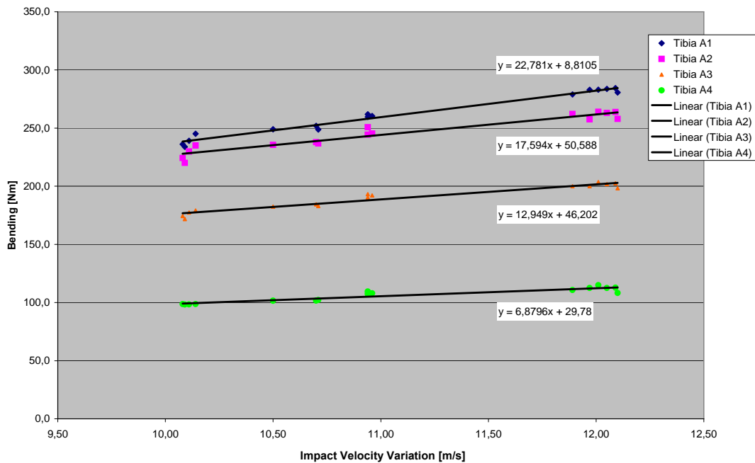
Fig. 15: Impact velocity variation: Tibia Bending Moments
