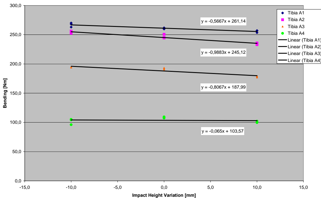
Fig. 13: Impact height variation: Tibia Bending Moments
