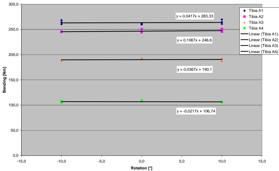
Fig. 11: Rotation around Z-axis: Tibia Bending Moments
