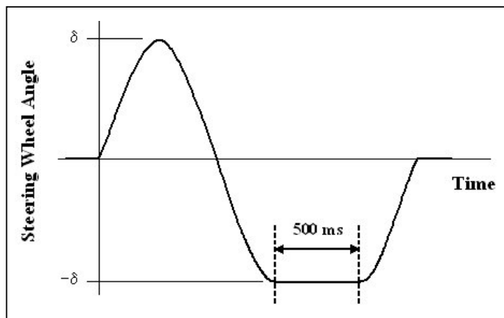
Figure 2. Sine with Dwell steering profile.
