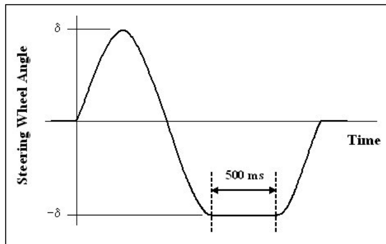
Figure 2. Sine with Dwell steering profile.
