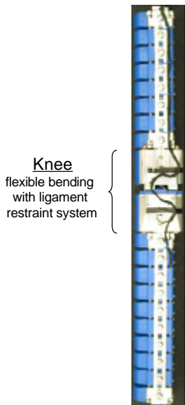
Flex-GT-prototype
