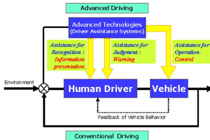
Figure 1 Block Diagram for Conventional and Advanced Driving
