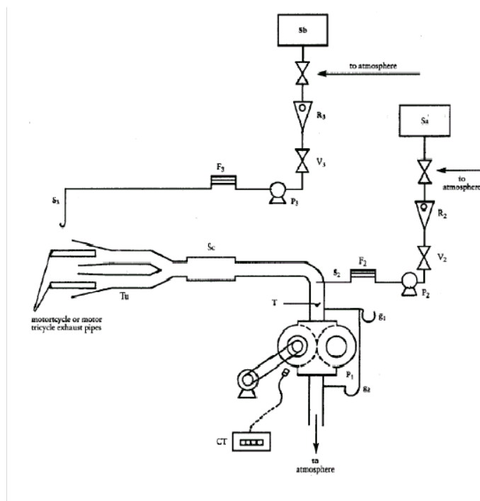
Figure 6-2: Equipment for sampling the gases and measuring their volume
