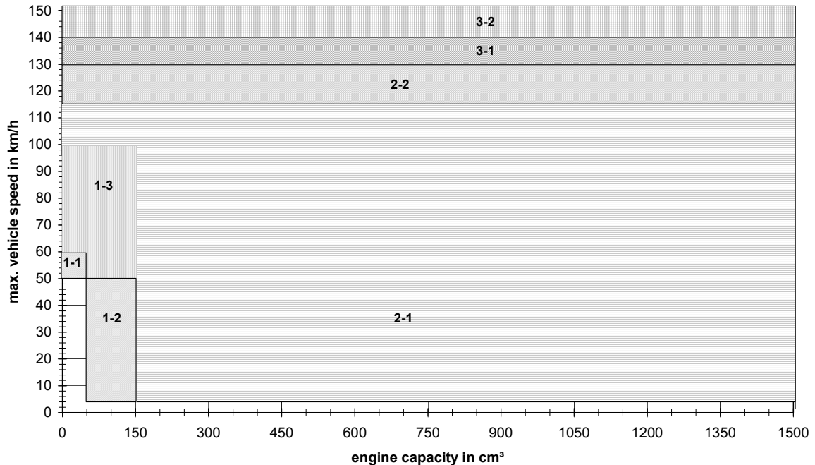
Figure 6-1: vehicle classification
