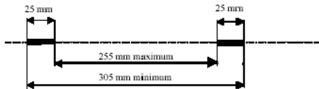
Figure 4: Distance between both low anchorage zones
